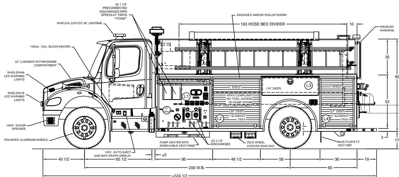
STREET SIDE VIEW
