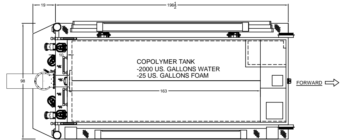
TOP VIEW (BODY)
